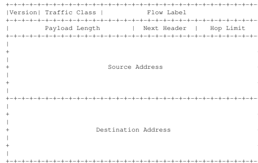
Figure 2.2: IPv6 Header, [16]
