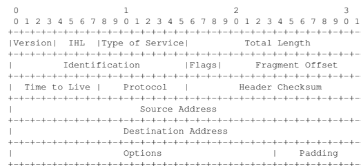
Figure 2.3: IPv4 Header, [38]
