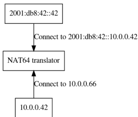
Figure 3.4: Network design
