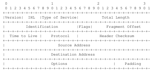
Figure 2.5: IPv4 Header [42]
