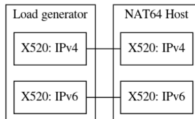
Figure 3.7: NAT64 in software benchmark
