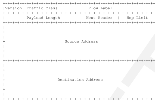
Figure 2.2: IPv6 Header, [15]
