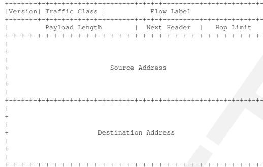
Figure 2.2: IPv6 Header, [15]
