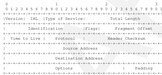
Figure 2.3: IPv4 Header, [37]
