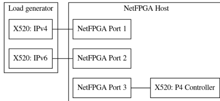
Figure 3.7: NAT64 with NetFPGA benchmark
