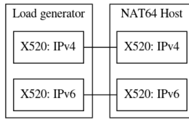
Figure 3.6: NAT64 in software benchmark
