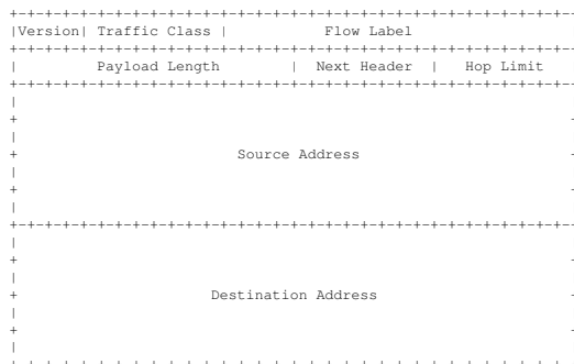
Figure 2.2: IPv6 Header [18]
