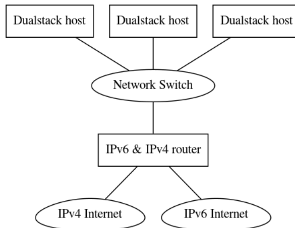
Figure 2.13: Dualstack network
