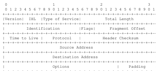
Figure 2.3: IPv4 Header [40]
