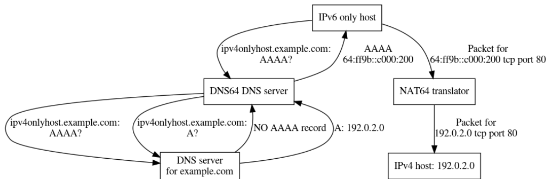
Figure 2.9: Illustration of DNS64
