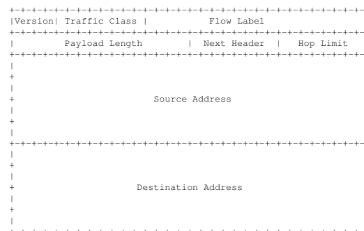
Figure 2.4: IPv6 Header [18]
