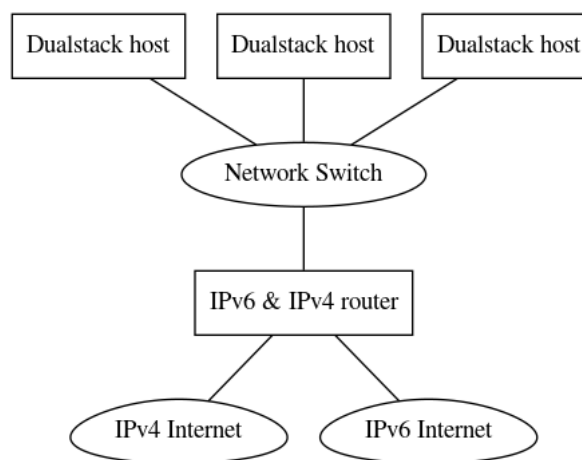
Figure 2.13: Dualstack network
