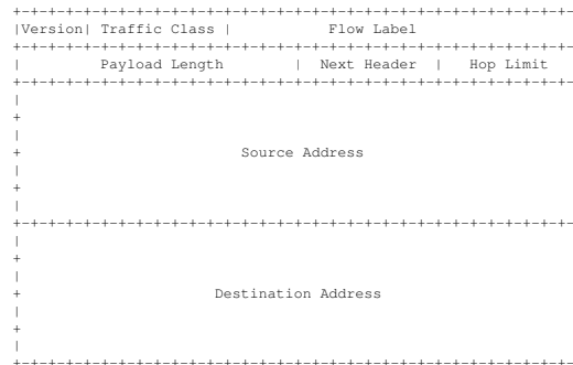
Figure 2.2: IPv6 Header [18]
