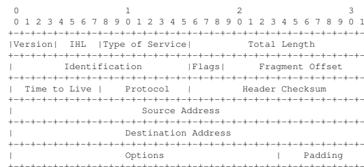
Figure 2.3: IPv4 Header [40]
