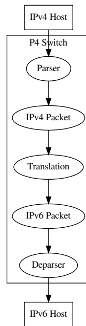
Figure 3.4: Our P4 Switch Architecture
