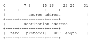
Figure 2.8: IPv4 Pseudo Header
