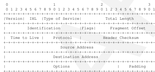
Figure 2.3: IPv4 Header, [36]
