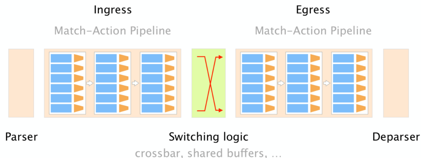
Figure 2.1: P4 protocol independence, [45]
