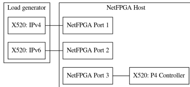
Figure 3.5: NAT64 with NetFPGA benchmark
