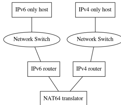
Figure 3.2: Standard NAT64 translation
