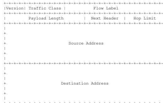
Figure 2.2: IPv6 Header [18]
