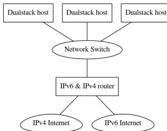
Figure 2.13: Dualstack network
