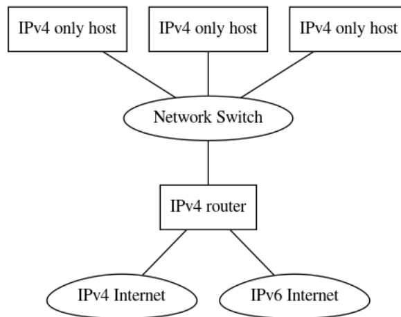
Figure 2.12: IPv4 only network
