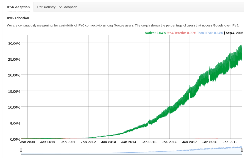
Figure 1.2: Google IPv6 Statistics, [21]
