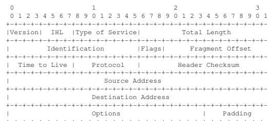
Figure 2.3: IPv4 Header [40]
