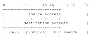
Figure 2.11: IPv4 Pseudo Header
