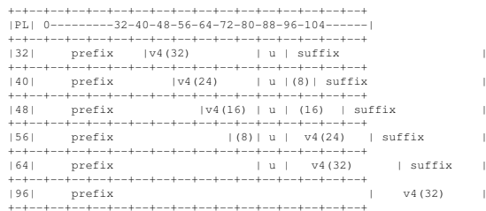
Figure 2.8: IPv4 embedding depending on the prefix length
