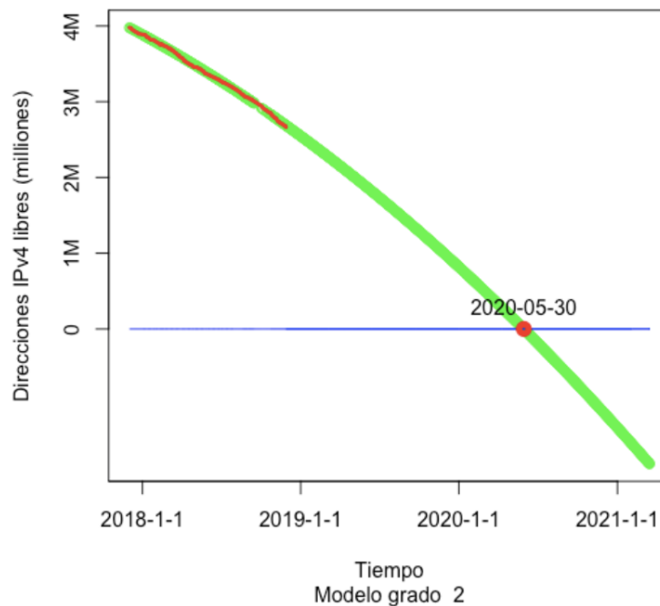
Figure 1.1: LACNIC Exhaustion projection, [26]
