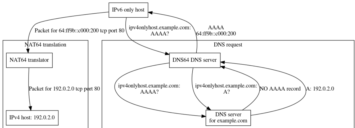
Figure 2.9: Illustration of DNS64
