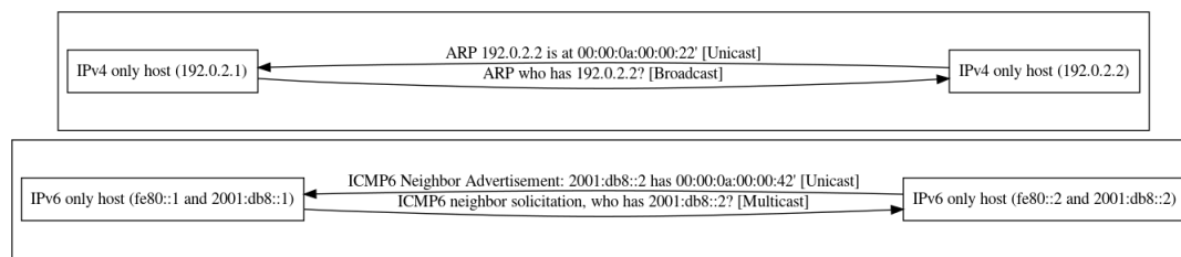
Figure 2.4: ARP and NDP
