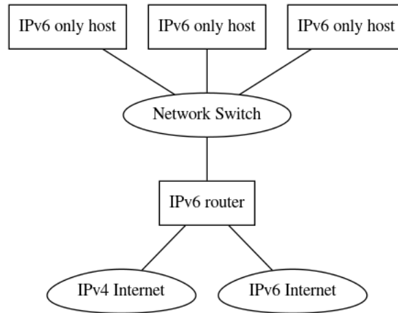
Figure 2.14: IPv6 only network
